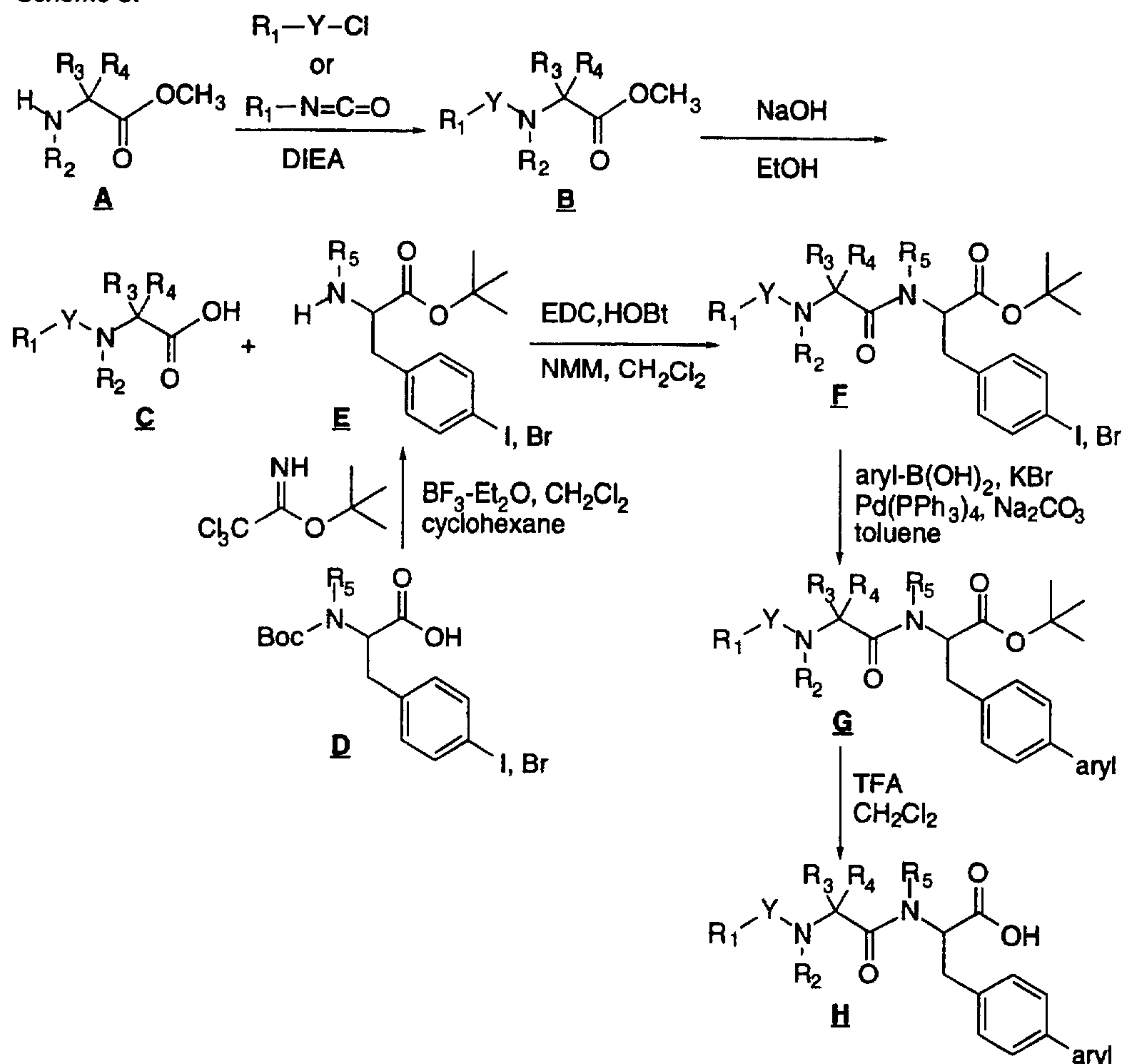
Scheme 3.
