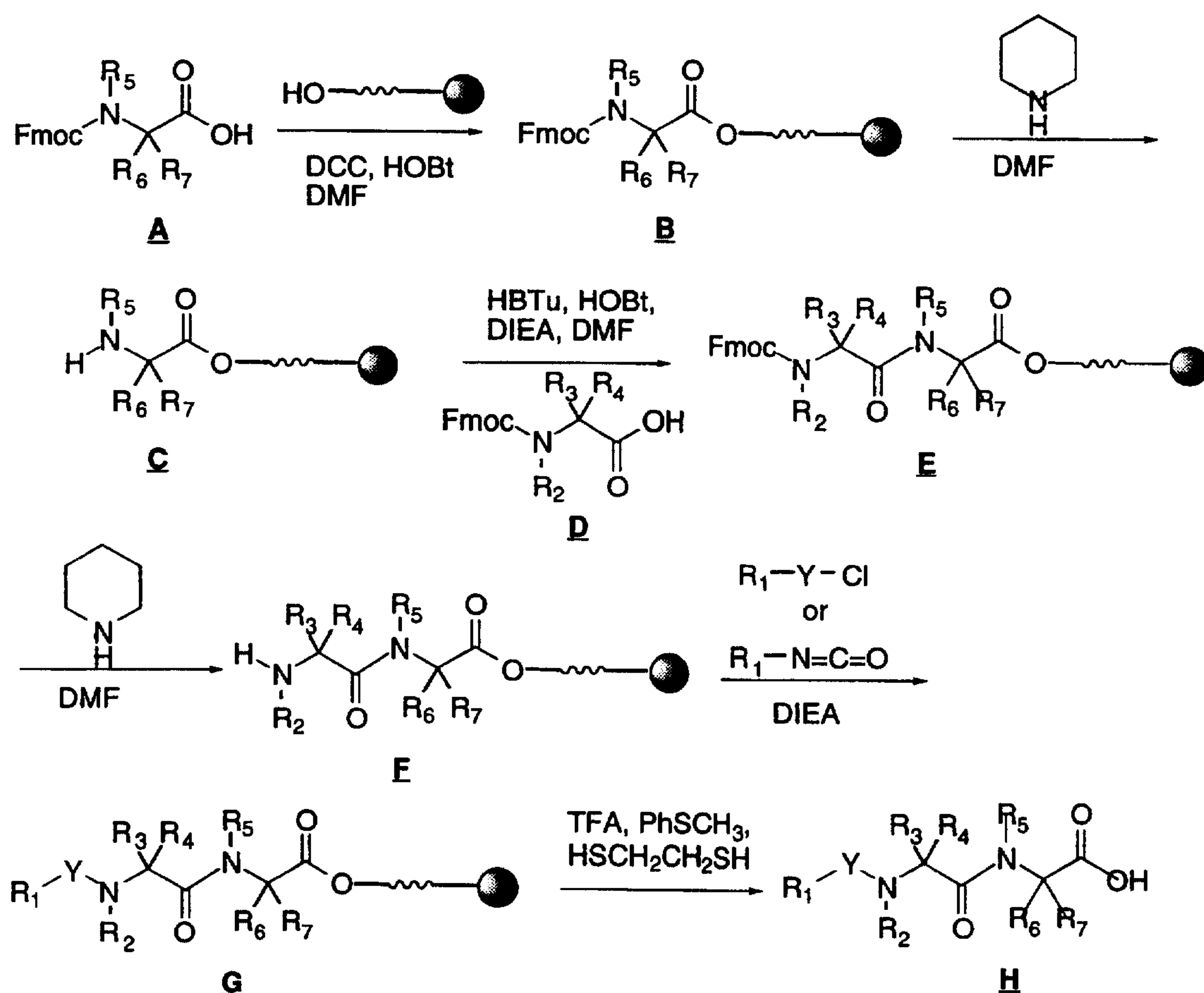
Scheme 1.
