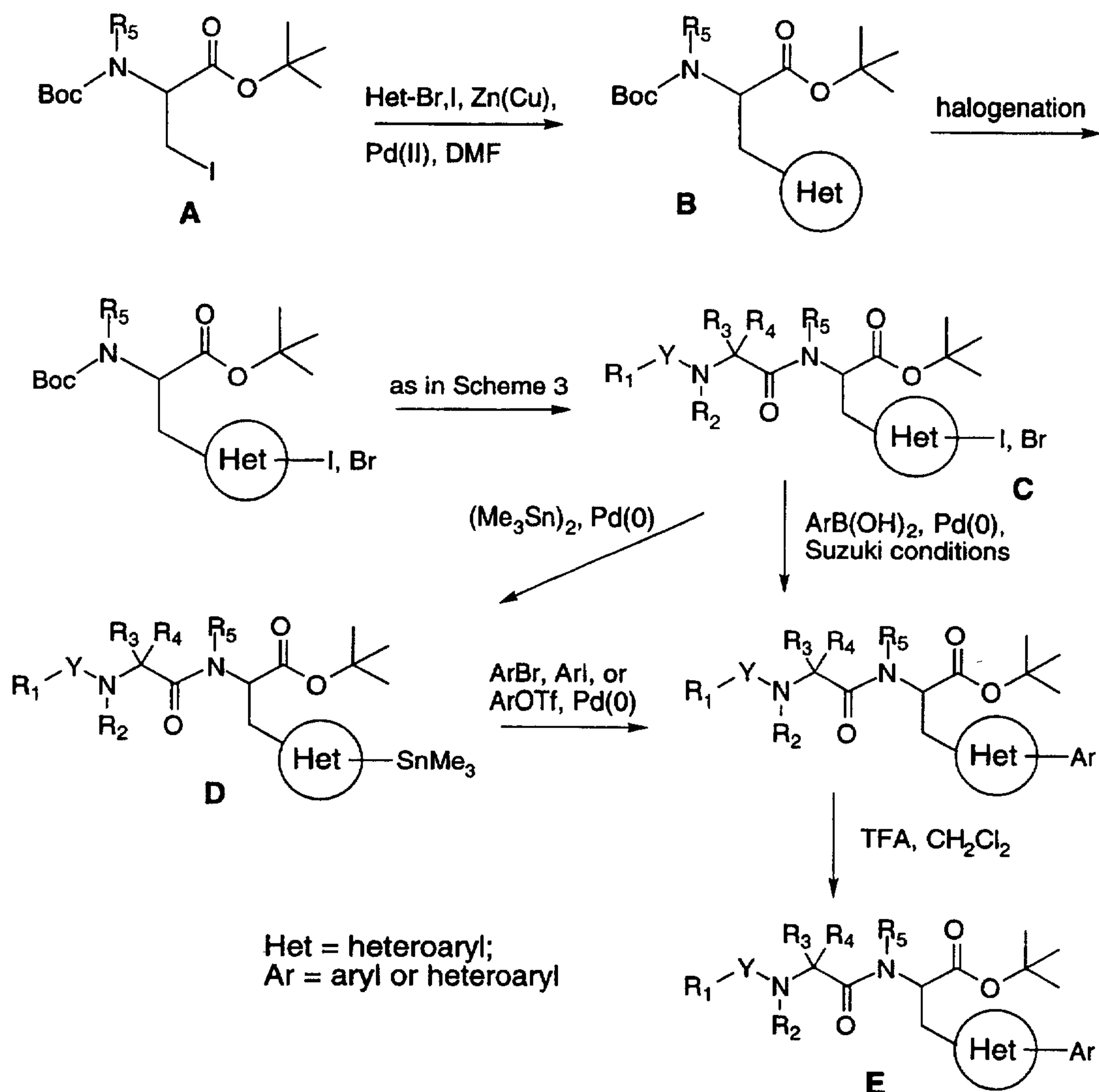
Scheme 5.
