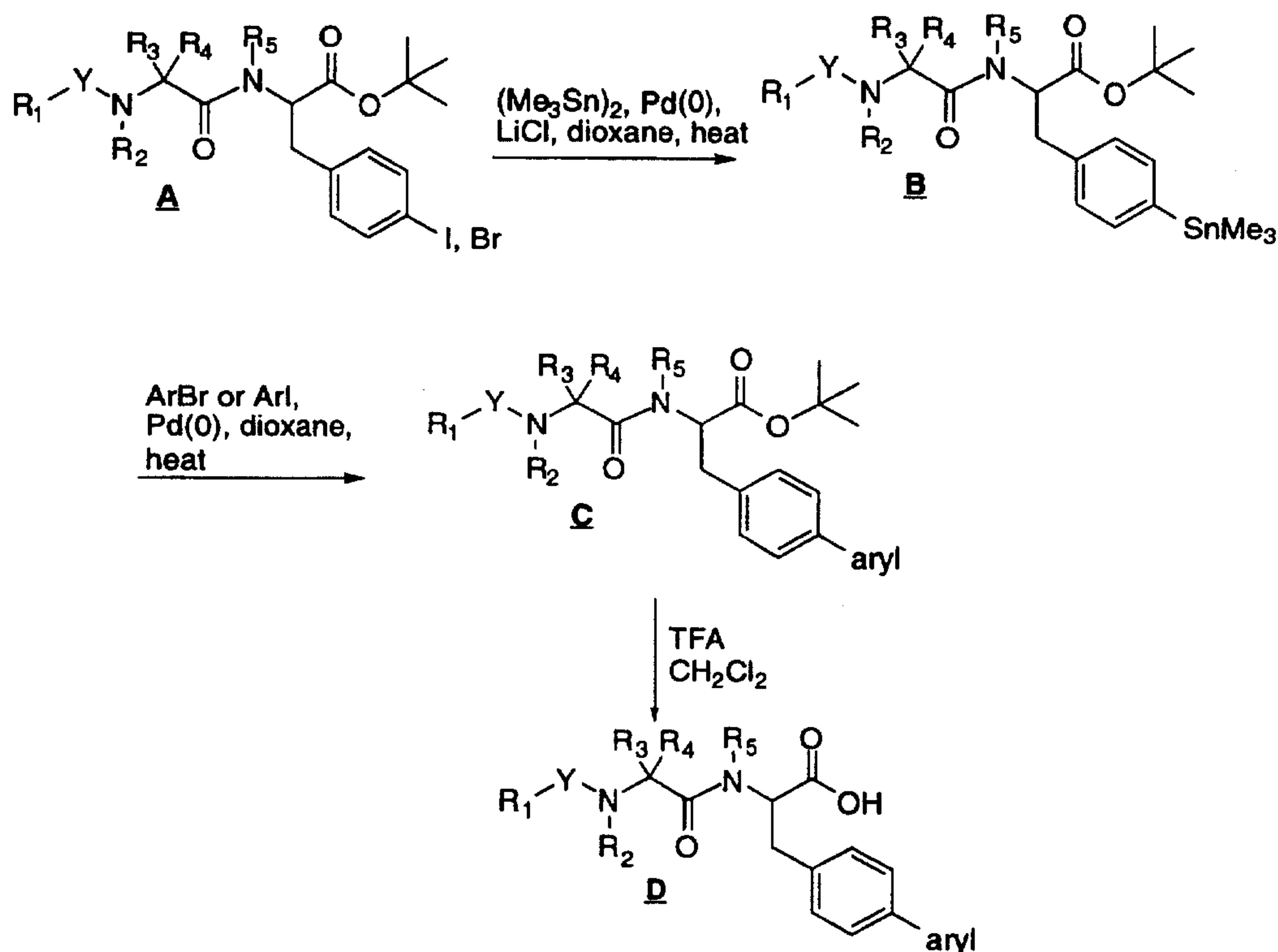
Scheme 4.
