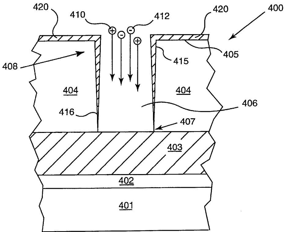
FIG. 3 (PRIOR ART)
