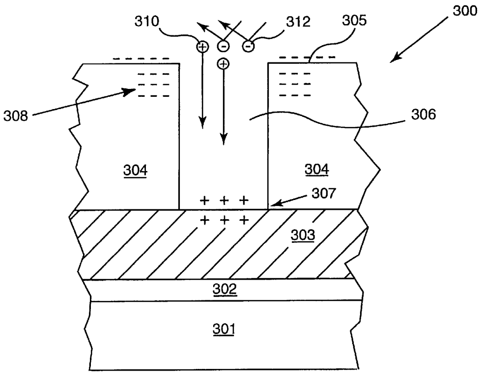
FIG. 3 (PRIOR ART)
