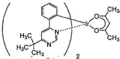
[Ir(tBuppm) 2 (acac)]
