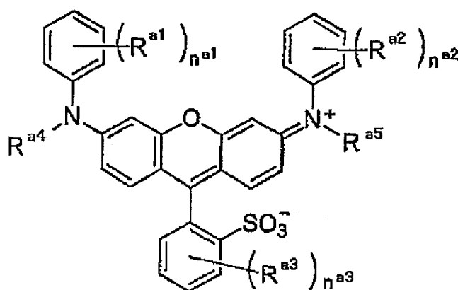
Formula (2)
