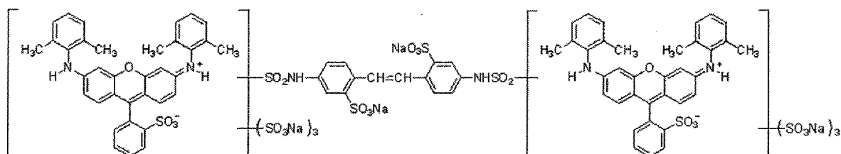
Exemplary Compound 1-4
