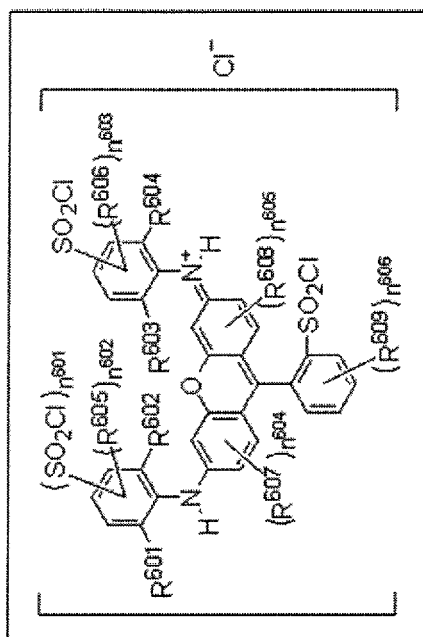
Formula (W9)
