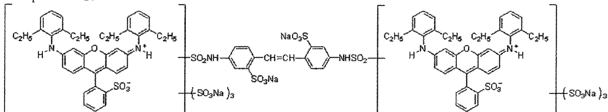
Exemplary Compound 1-17
