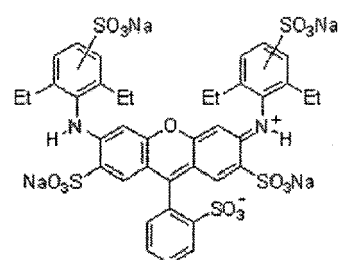
Exemplary Compound (6)
