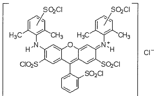
Compound A:
