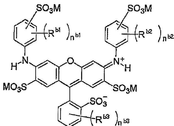
Formula (3)
