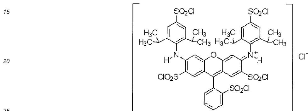
Compound C
