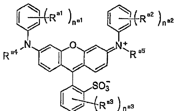
Formula (2)
