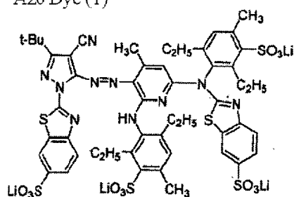
Azo Dye (1)
