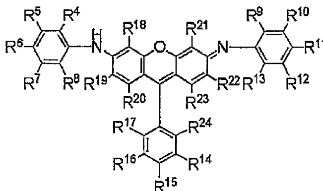
Formula (5)
