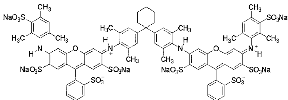
[0199] Exemplary Compound 1-16:
