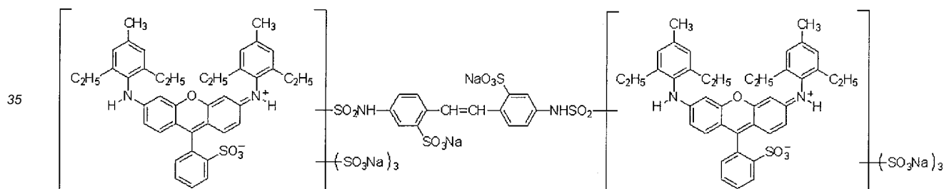
Compound D
