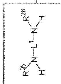
Formula (W10)
