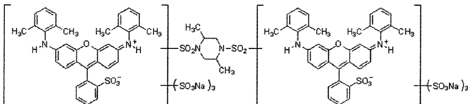
Exemplary Compound 1-17
