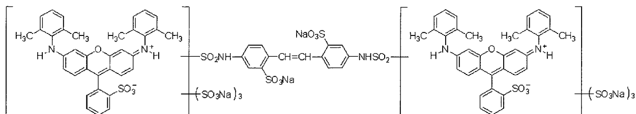
Compound A:
