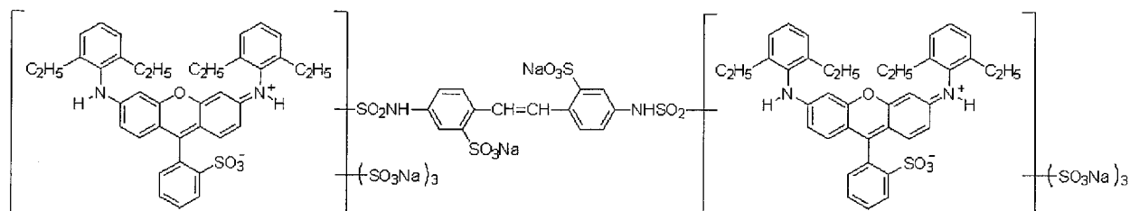
Compound B
