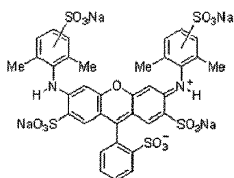
Exemplary Compound (1)
