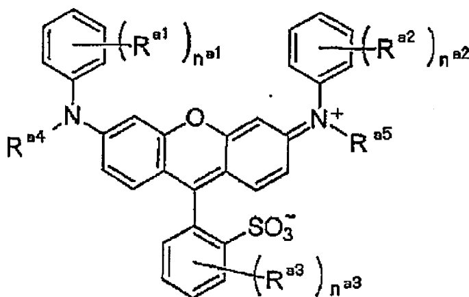
Formula (2)
