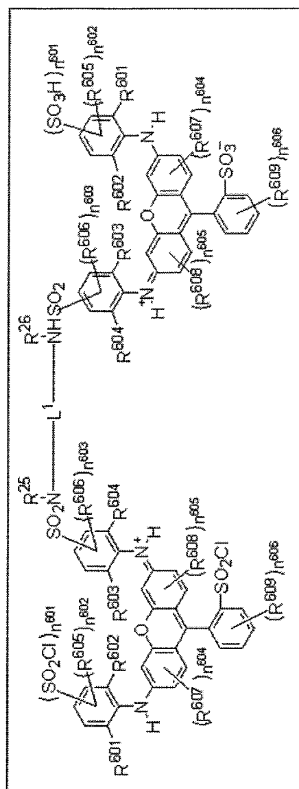
Formula (W11)
