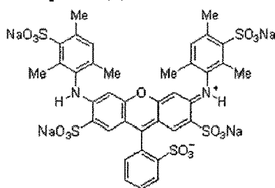
Exemplary Compound (4)
