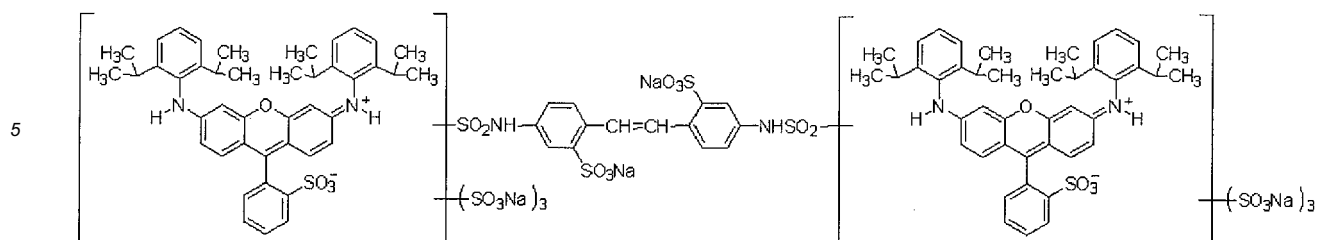
Compound C
