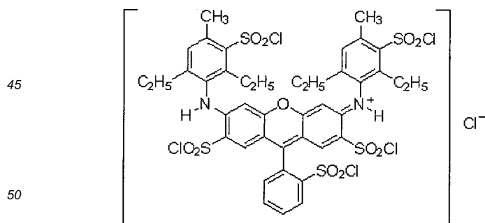
Compound D
