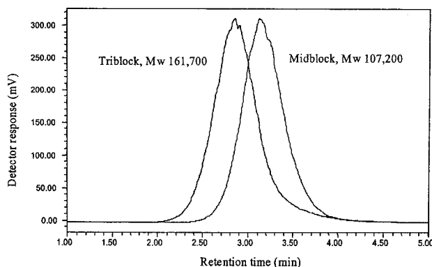
SEC traces of midblock and triblock polymers
