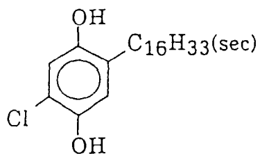
(Cpd-10) Additive
