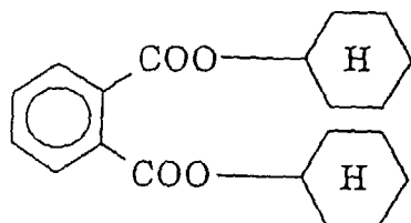
Solvent (Solv-6)
