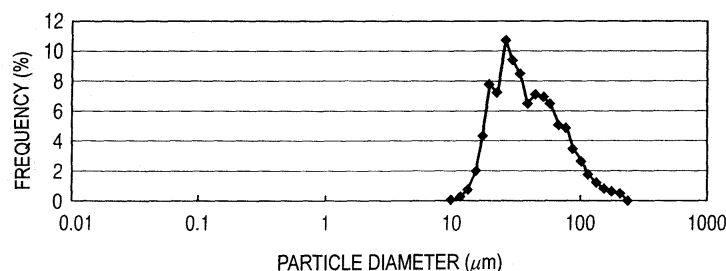
PARTICLE SIZE DISTRIBUTION OF FINE SILICA POWDER A
