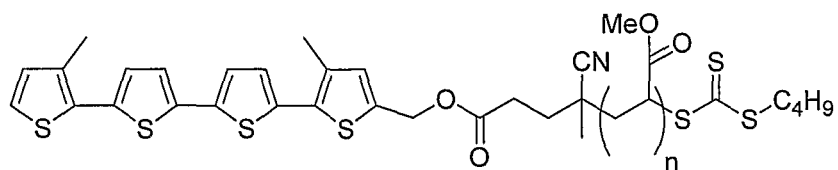
4MT-PMA-RAFT
