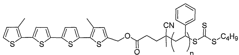
4MT-PS-RAFT
