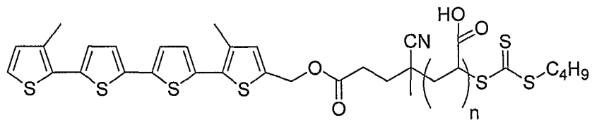
4MT-PAA-RAFT
