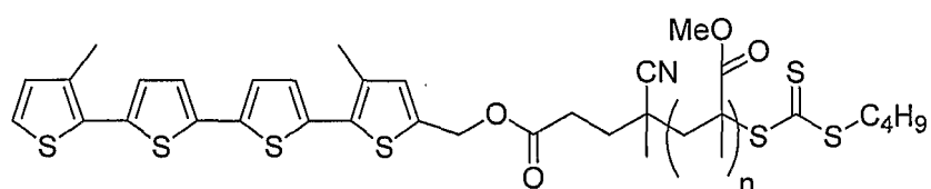
4MT-PMMA-RAFT
