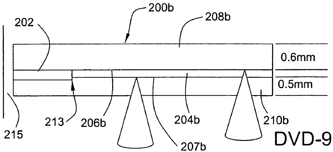
Single-Sided Double Layer Disc
