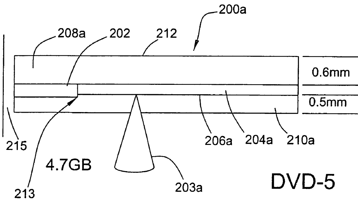
FIG. 2A Single-Sided, Single Layer Disc
