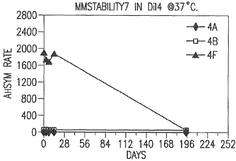
FIG.3D
