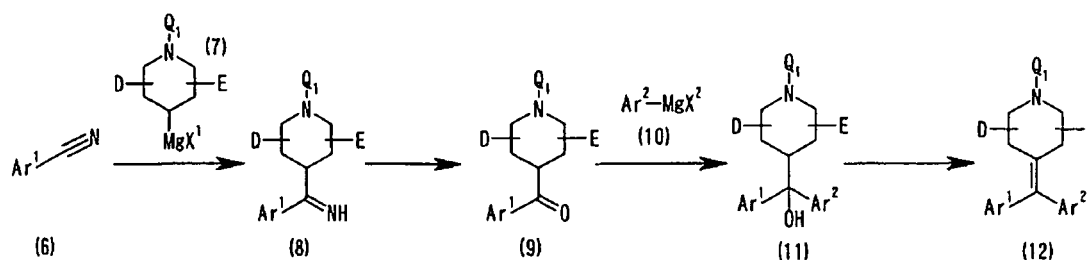
Reaction scheme 1
