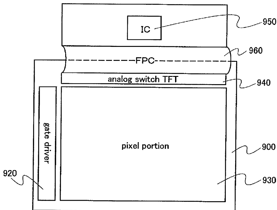
FIG. 17A IC connected by FPC
