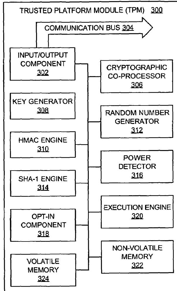
FIG. 3 (PRIOR ART)
