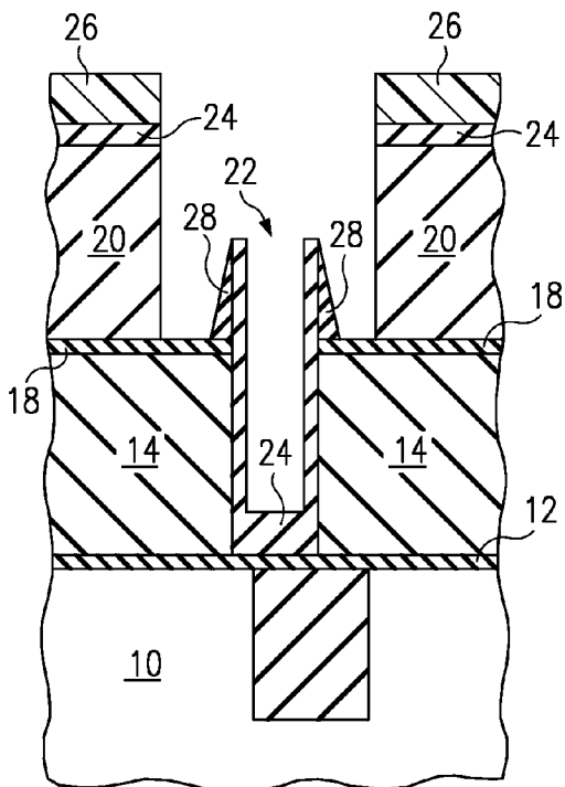
FIG. 1D (PRIOR ART)
