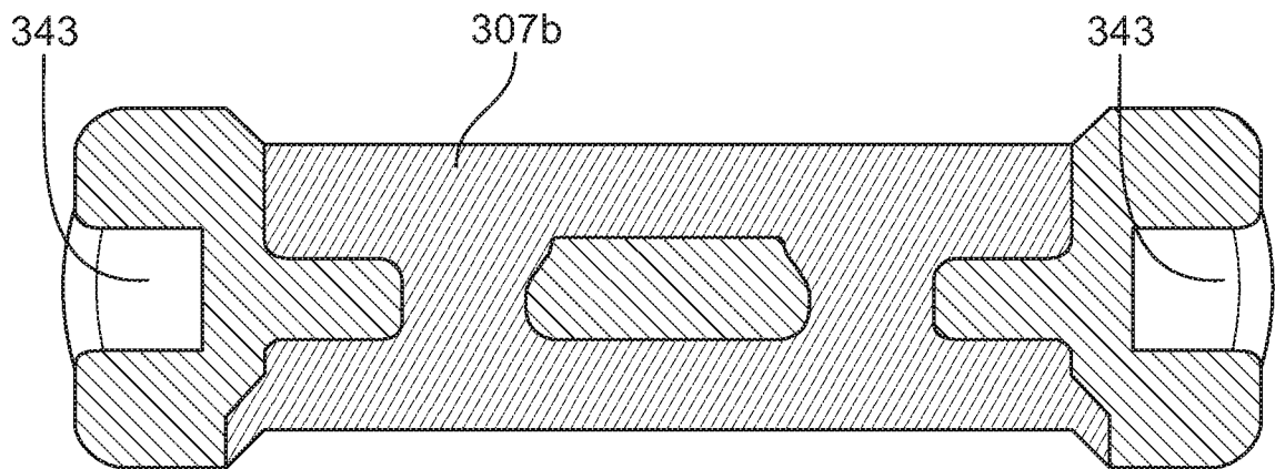
SECTION F-F
