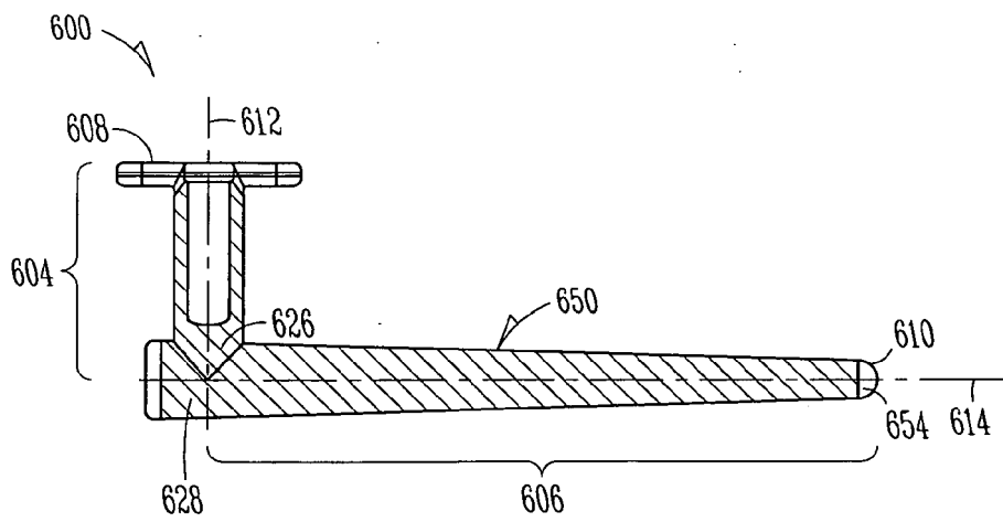
SECTION 6B-6B
