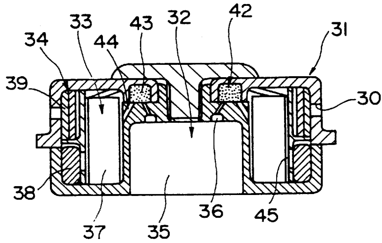
Fig. 6 (CONVENTIONAL ART)
