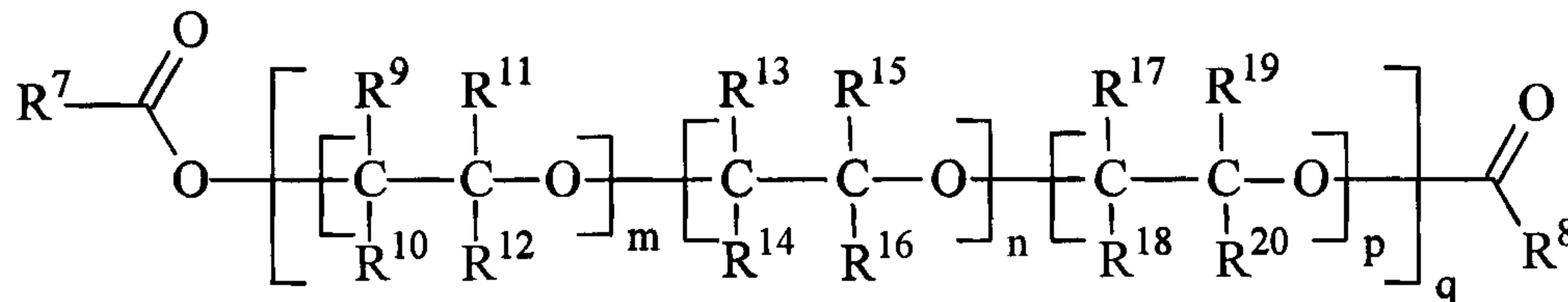
Formula (2)
