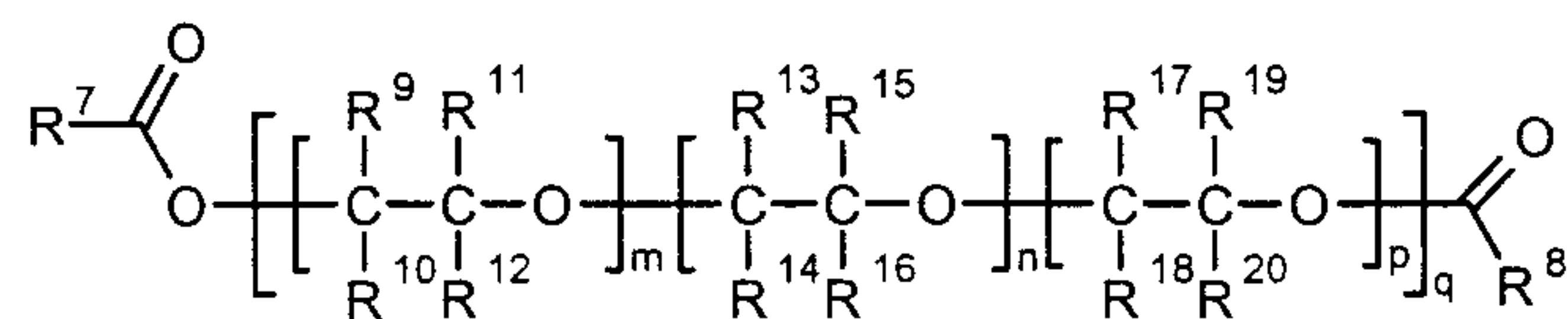
Formula (2)
