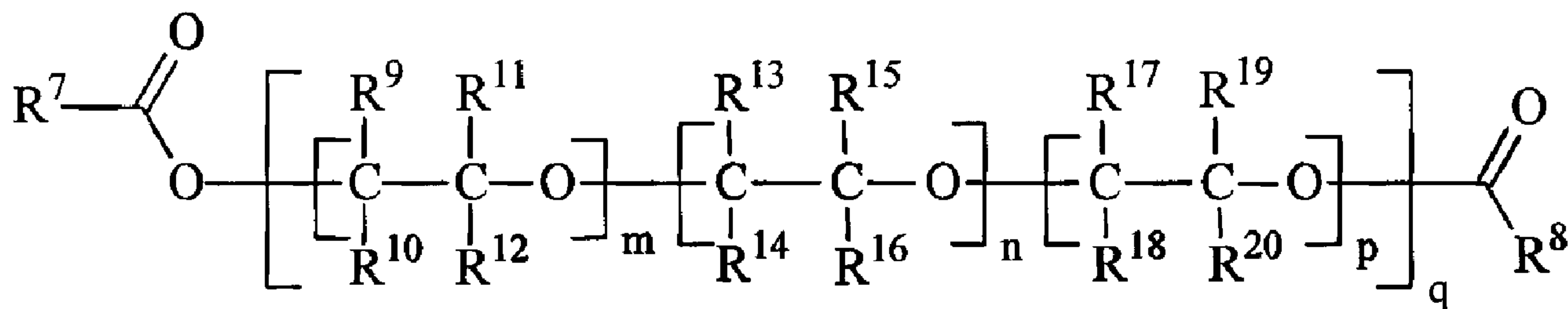
Formula (2)
