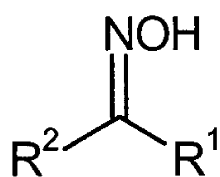
Formula (1)
