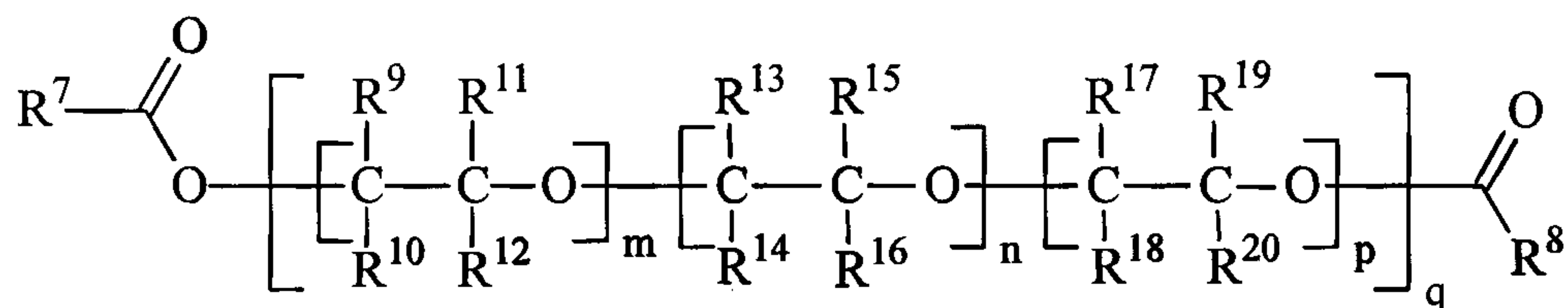
Formula (2)
