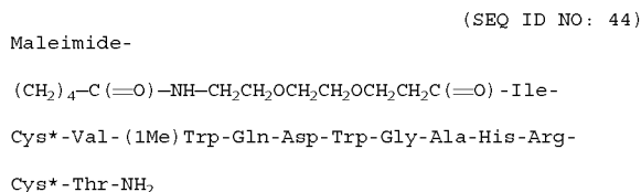
Compound III
