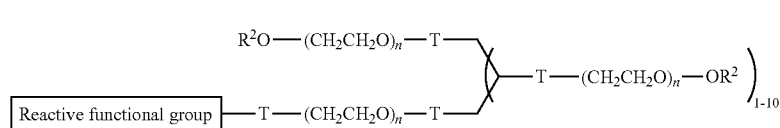
Formula F
