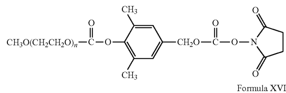
Formula XVI
