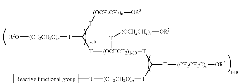
Formula H
