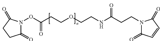
Compound III
