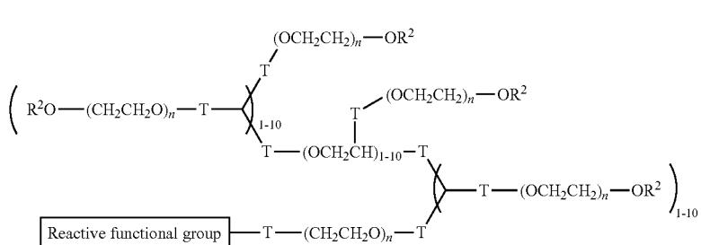
Formula G
