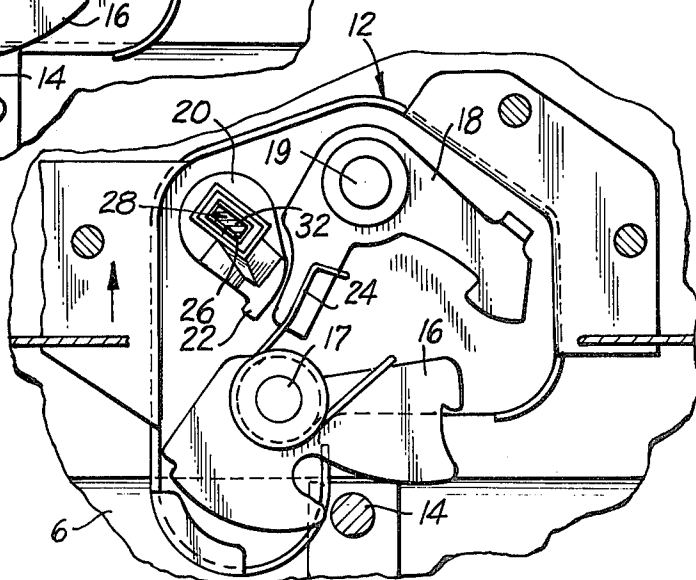
Fig. 3. UNLOCKED
