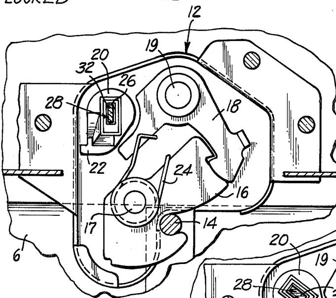
Fig. 2. LOCKED
