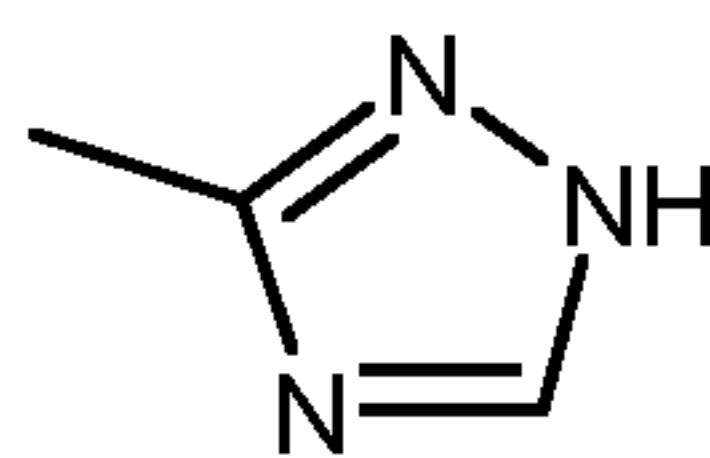
2H-tautomer
