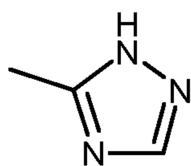
1H-tautomer
