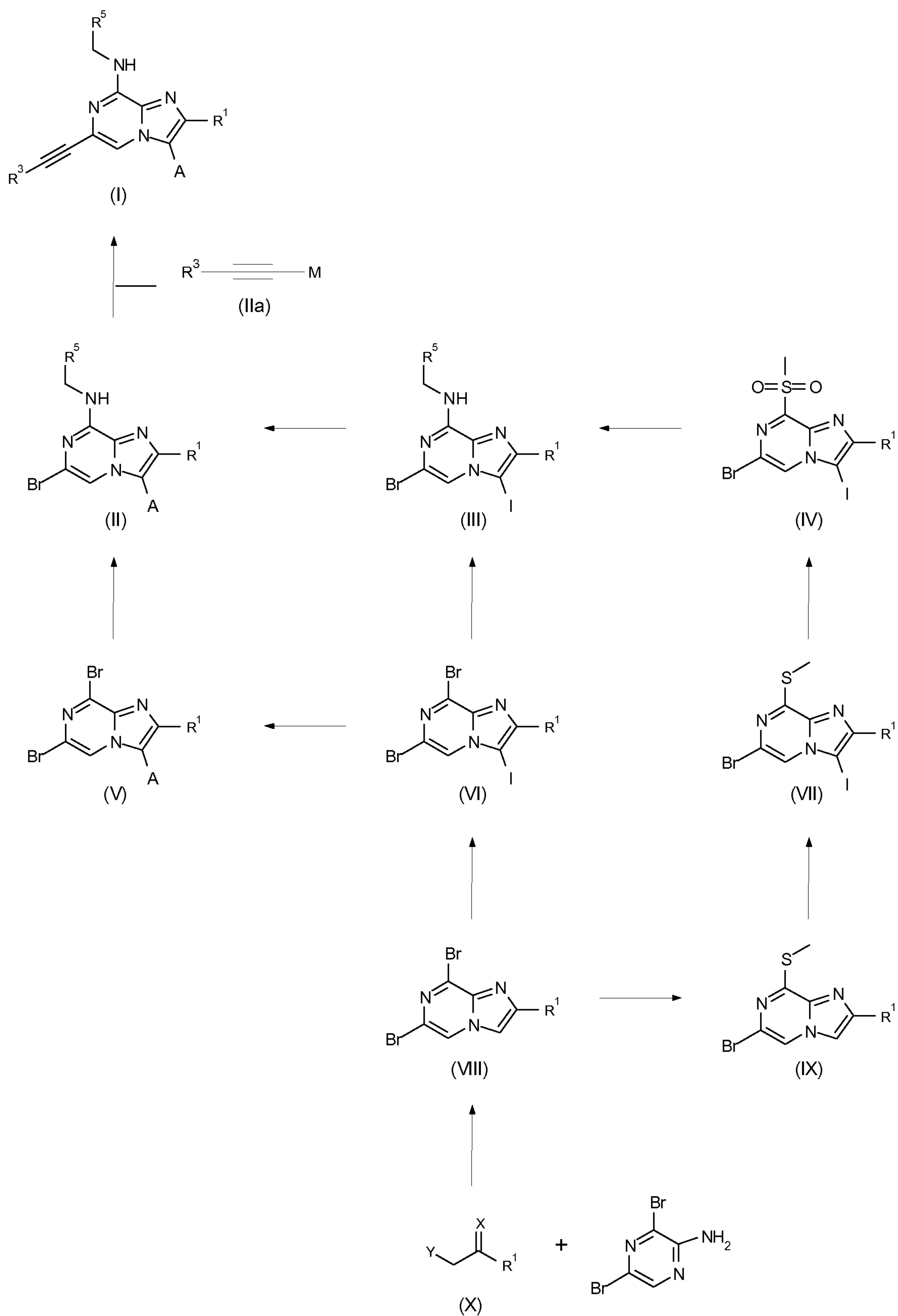
Scheme 1
