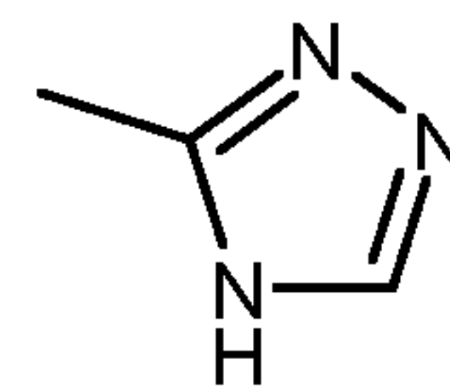
4H-tautomer.
