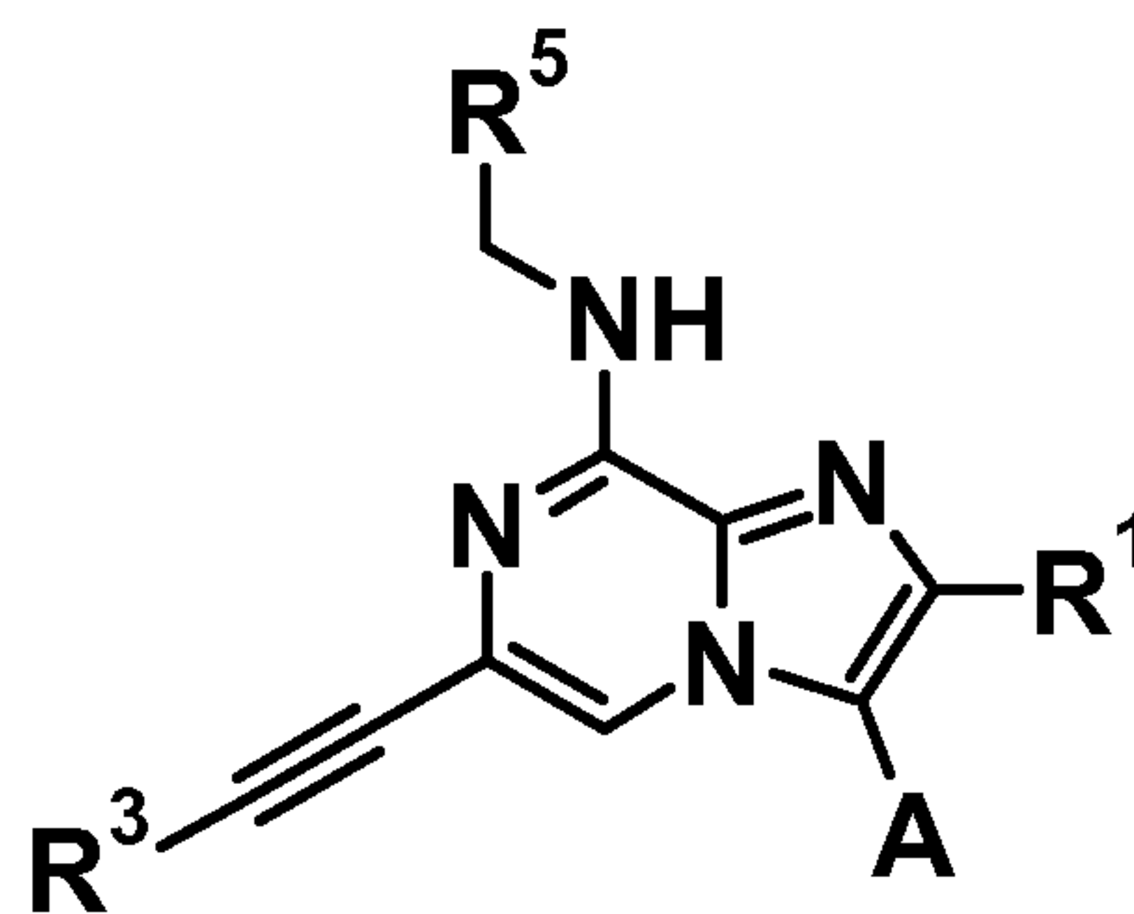
(I)
