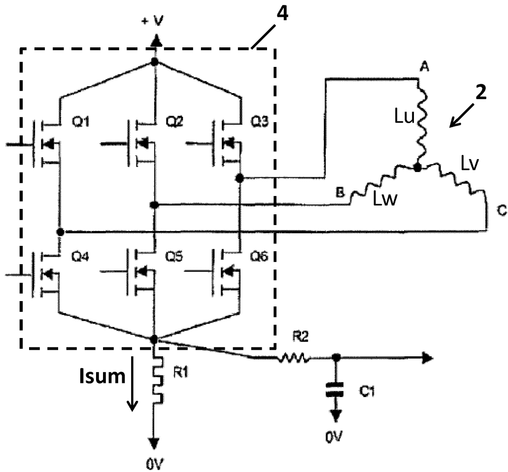
FIG. 3 (prior art)
