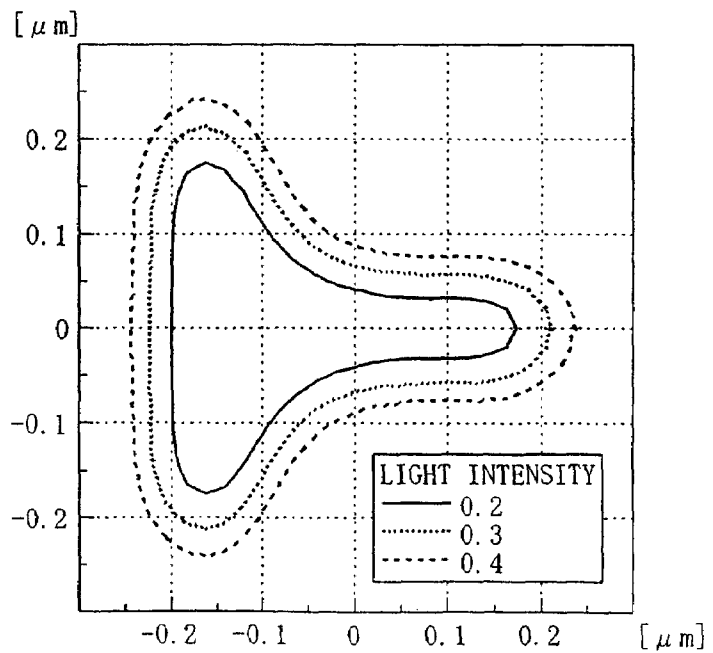
Fig. 33(b) Prior Art
