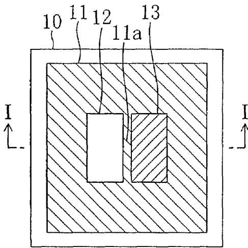
Fig. 34(a) Prior Art
