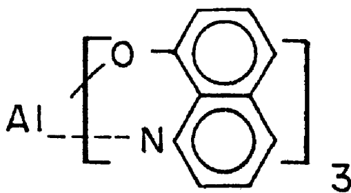
tris(8-hydroxyquinoline) aluminium
