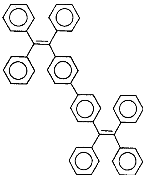
4,4'-bis [(1,2,2-trisphenyl)ethenyl] -biphenyl
