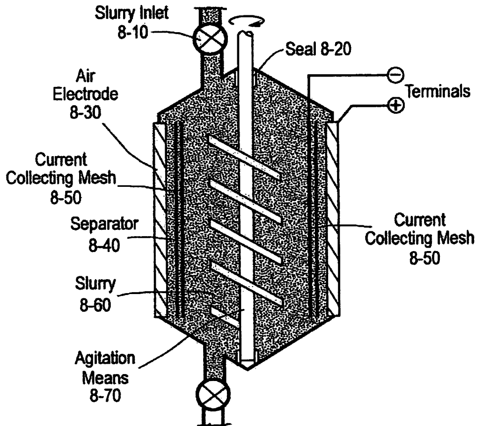
Fig.8 Side View Schematic
