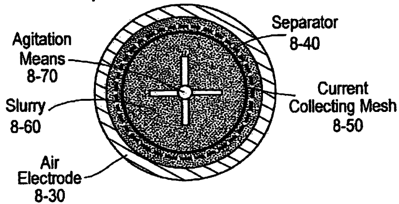
Top View Schematic
