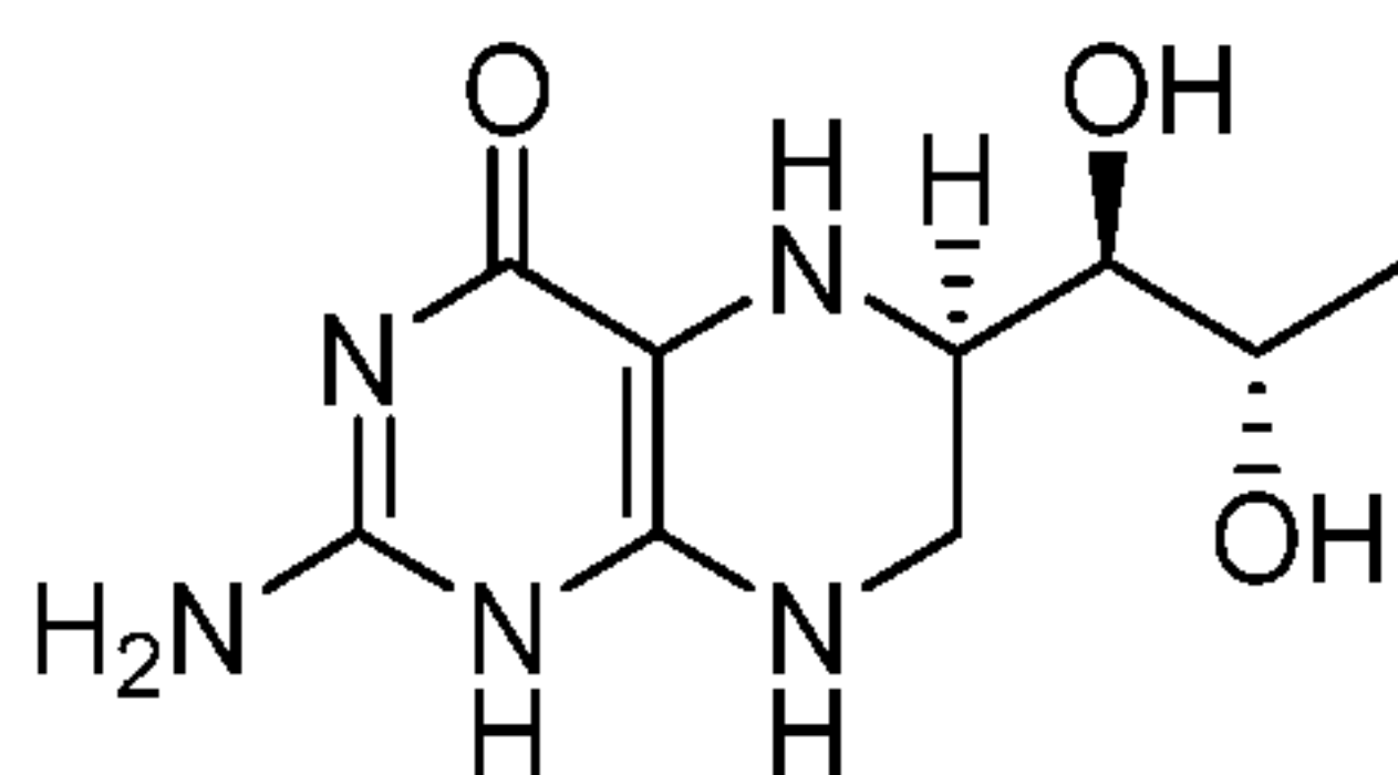
Tetrahydrobiopterin
