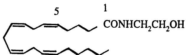
Arachidonylethanolamide (anandamide)
