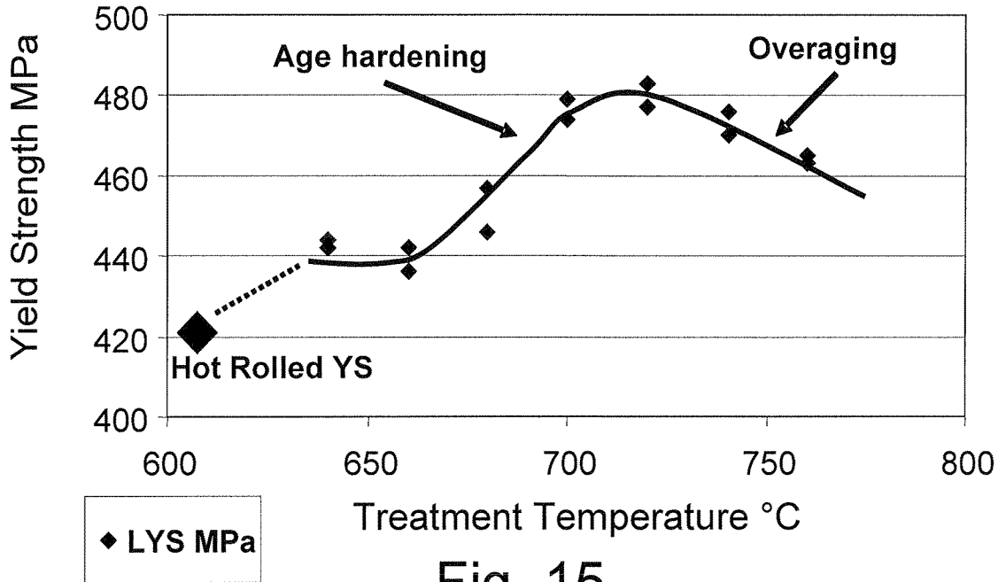
Laboratory Heat Treatment of a 0.026% Nb steel for 10 Seconds Hold at Peak Temperature
