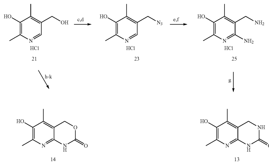
Scheme 2. Synthesis of pyridinol-fused ring analog 13.
