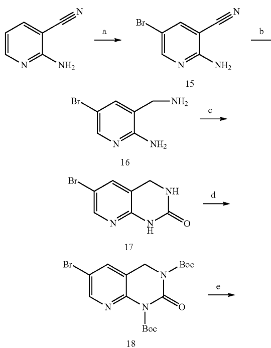
Scheme 1. Synthesis of pyridinol-fused ring analog 12.
