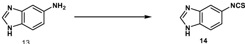
Scheme 4: Synthesis of 5-isothiocyanato-1H-benzo[d]imidazole (14)
