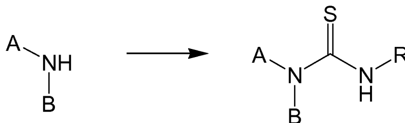
5 Scheme 1: Synthesis of the thiourea derivatives
