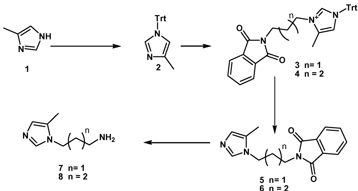
Scheme 2: Synthesis of the 3-(5-methyl-1H-imidazol-1-yl)alkyl-1-amines ( 7 and 8 )
