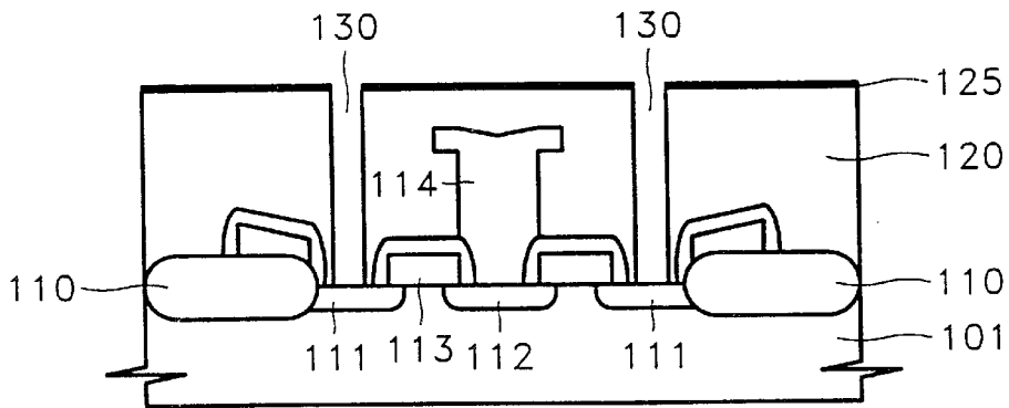
FIG. 2 (PRIOR ART)
