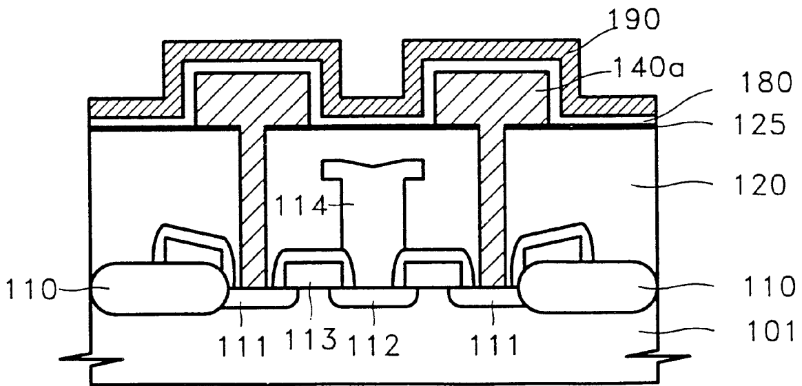
FIG. 5 (PRIOR ART)
