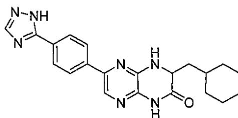
6-(4-(1H-1,2,4-triazol-5-yl)phenyl)-3-(cyclohexylmethyl)-3,4-dihydropyrazino[2,3-b]pyrazin-2(1H)-one;
