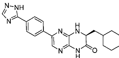
(R)-6-(4-(1H-1,2,4-triazol-5-yl)phenyl)-3-(cyclohexylmethyl)-3,4-dihydropyrazino[2,3-b]pyrazin-2(1H)-one.
