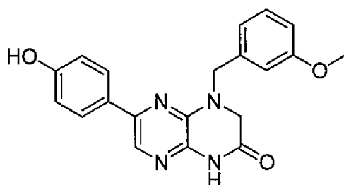
6-(4-hydroxyphenyl)-4-(3-methoxybenzyl)-3,4-dihydropyrazino[2,3-b]pyrazin-2(1H)-one;
