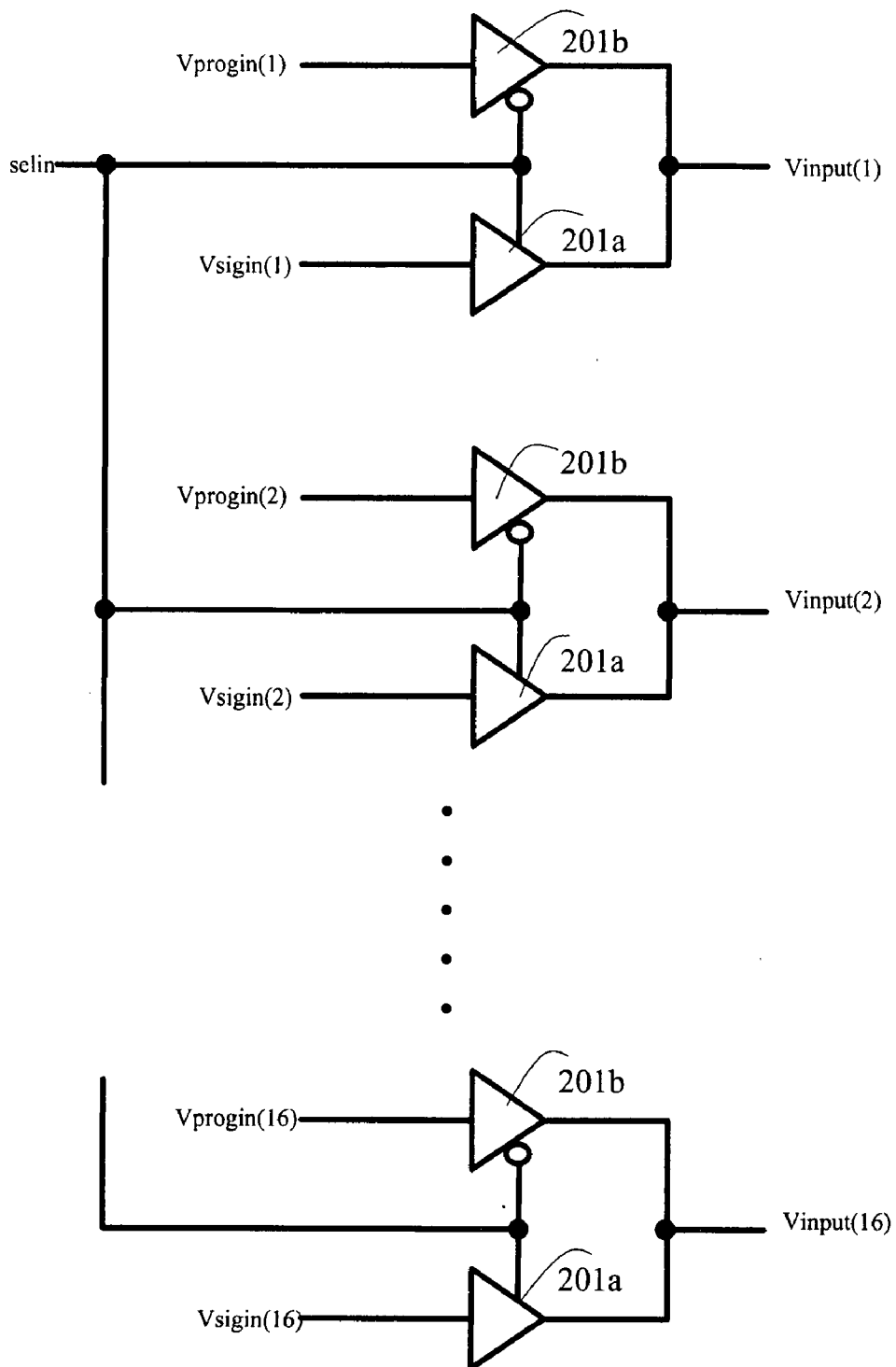
Fig.2 Input Selector Circuit
