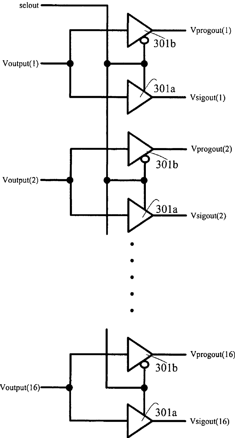
Fig.3 Output Selector Circuit
