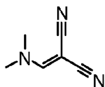
18 D (Dimethylaminomethylene)malononitrile
