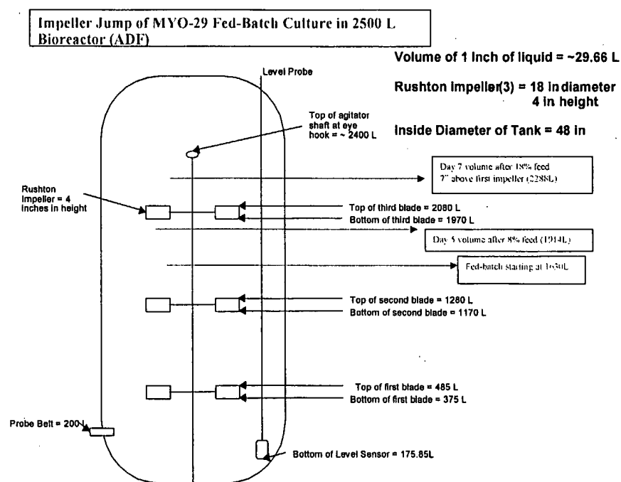
Figure 24. Impeller Jump
