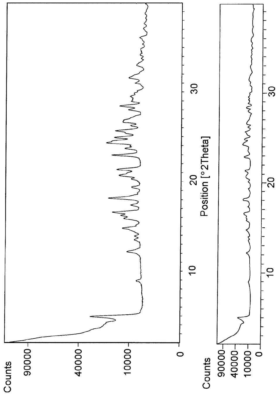
FIG. 2 XRPD of Polymorph A of Compound A
