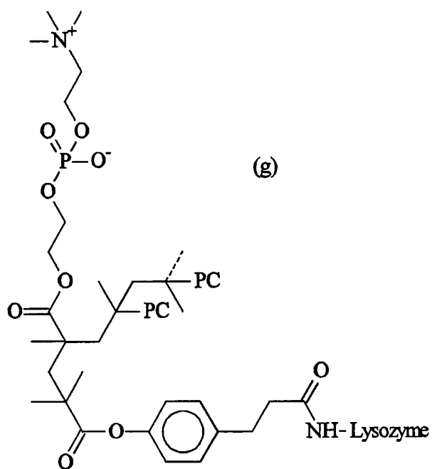
Example 10.3 - ATRP using the lysozyme conjugated initiator.
