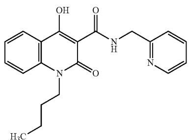
1-butyl-4-hydroxy-2-oxo-N-(2-pyridinylmethyl)-1,2-dihydro-3-quinolinecarboxamide
