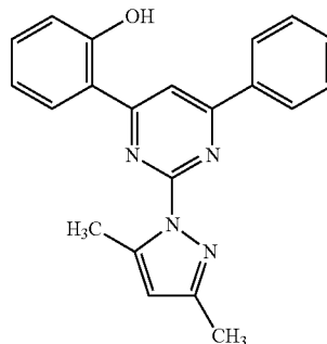
2-[2-(3,5-dimethyl-1H-pyrazol-1-yl)-6-phenyl-4-pyrimidinyl]phenol
