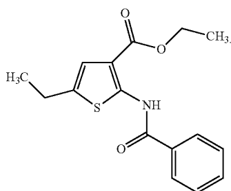
ethyl 2-(benzoylamino)-5-ethyl-3-thiophenecarboxylate
