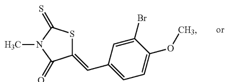
5-(3-bromo-4-methoxybenzylidene)-3-methyl-2-thioxo-1,3-thiazolidin-4-one
