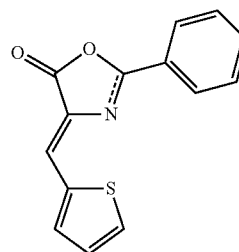
2-phenyl-4-(2-thienylmethylene)-1,3-oxazol-5(4H)-one
