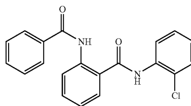
2-(benzoylamino)-N-(2-chlorophenyl)benzamide
