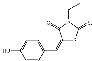
3-ethyl-5-(4-hydroxybenzylidene)-2-thioxo-1,3-thiazolidin-4-one
