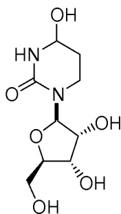
Tetrahydrouridine (THU)
