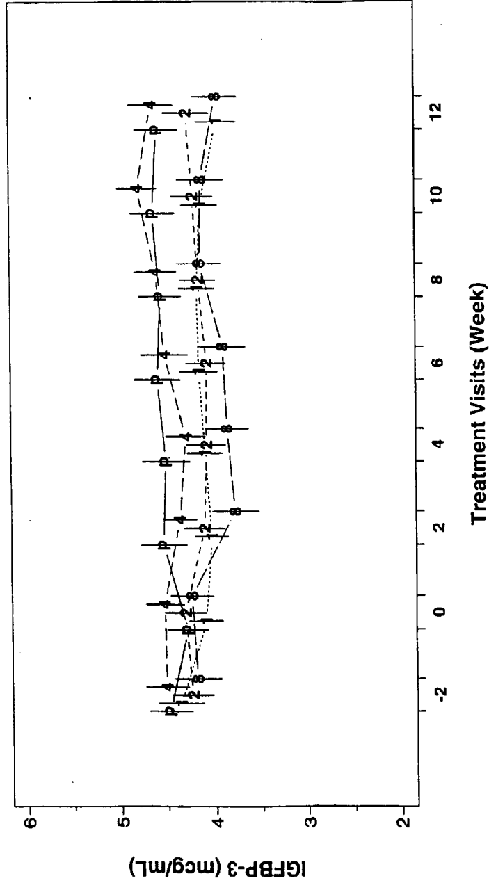
Effect of IGF-I Treatment on IGFBP-3 (Mean \pm SE)
