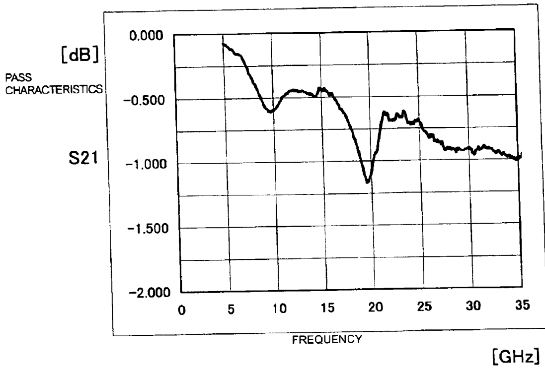
FIG. 19 PRIOR ART
