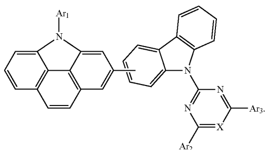
Formula 2
