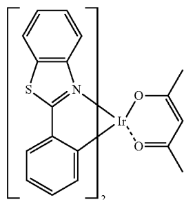
Ir(BT) 2 (acac)
