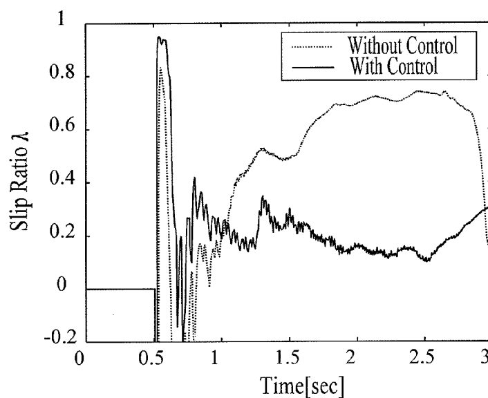
COMPARISON OF SLIP RATIO
