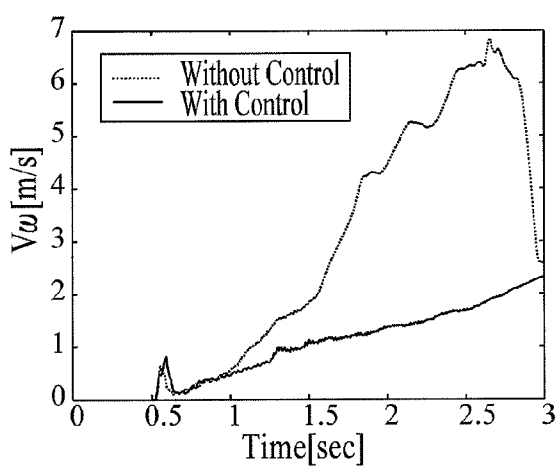
COMPARISON OF WHEEL SPEED
