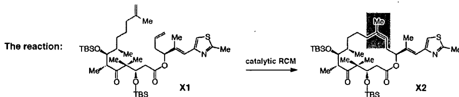
Scheme X1. Initial Screening of Mo and W Complexes to Promote Formation of 2 through Macroscopic RCM
