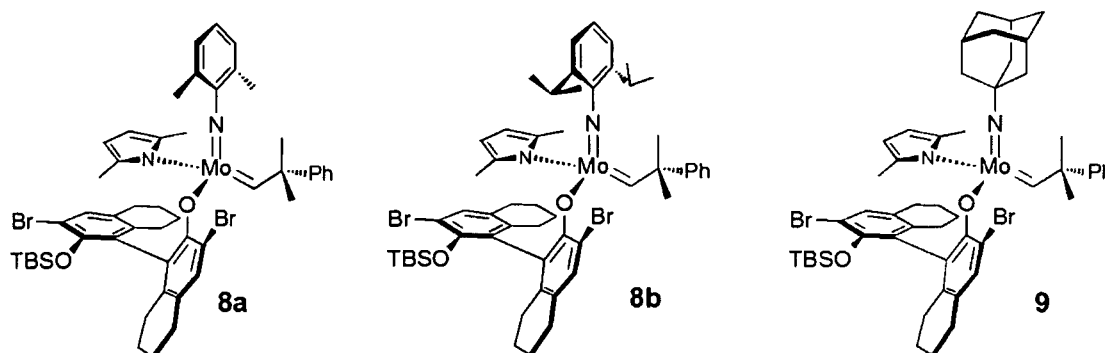
Chart 2. In situ Generated Mo Monoalkoxide-monopyrrolide Complexes.
