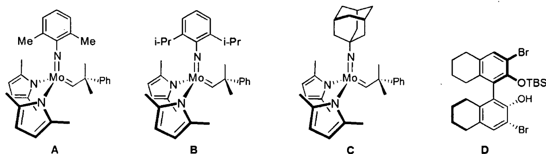
Chart 1. Mo Bis-pyrrolide Complexes and Chiral Enantiomerically Pure Alcohol.
