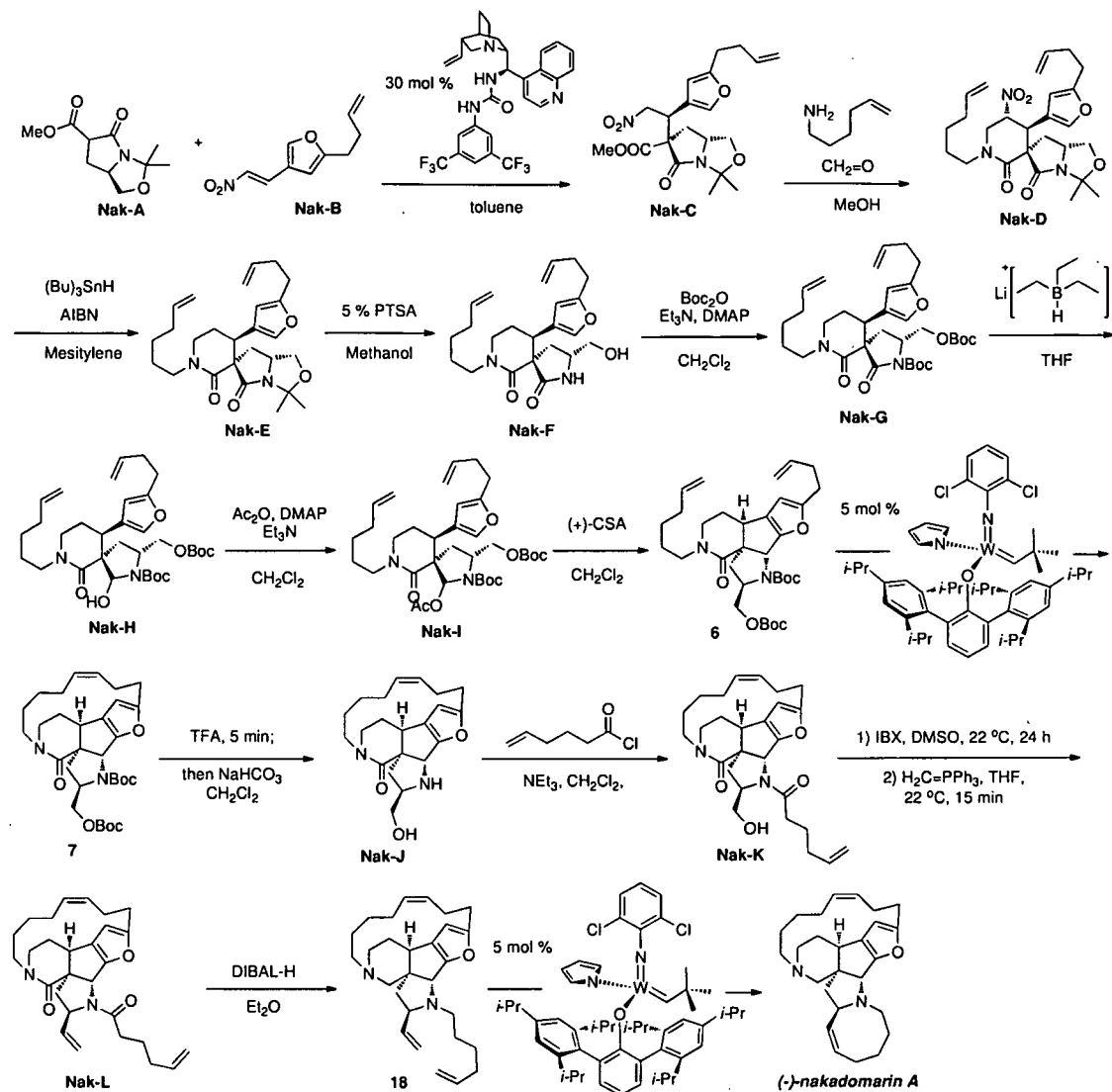
Chart 3. Synthesis of (-)-Nakadamarin A.
