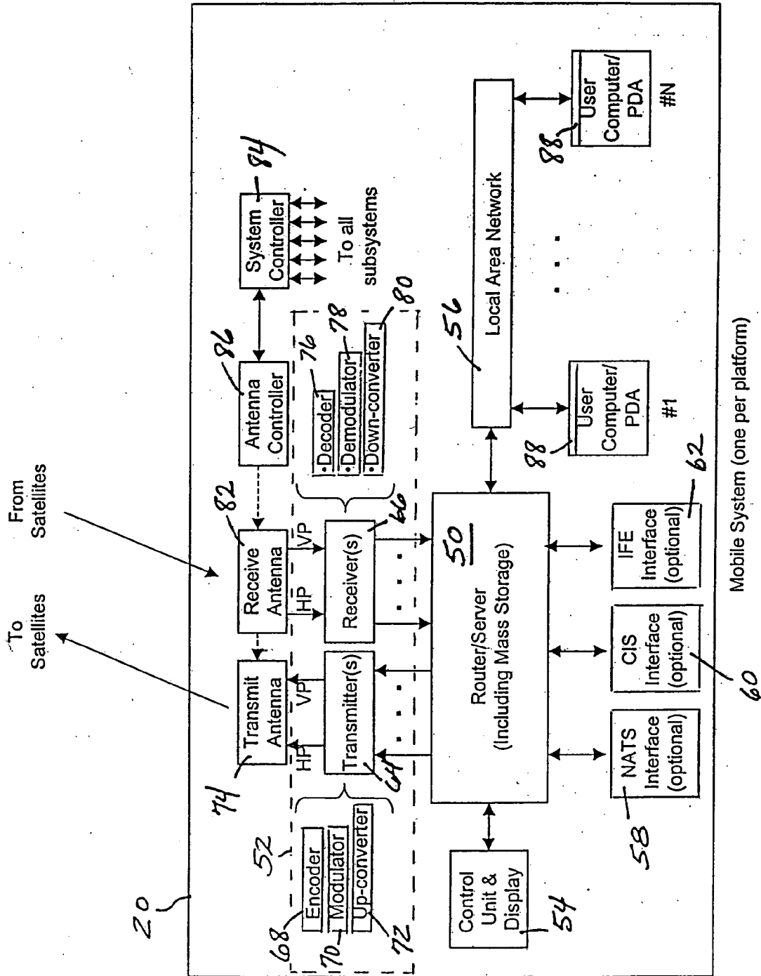
Fig. 2 Mobile System
