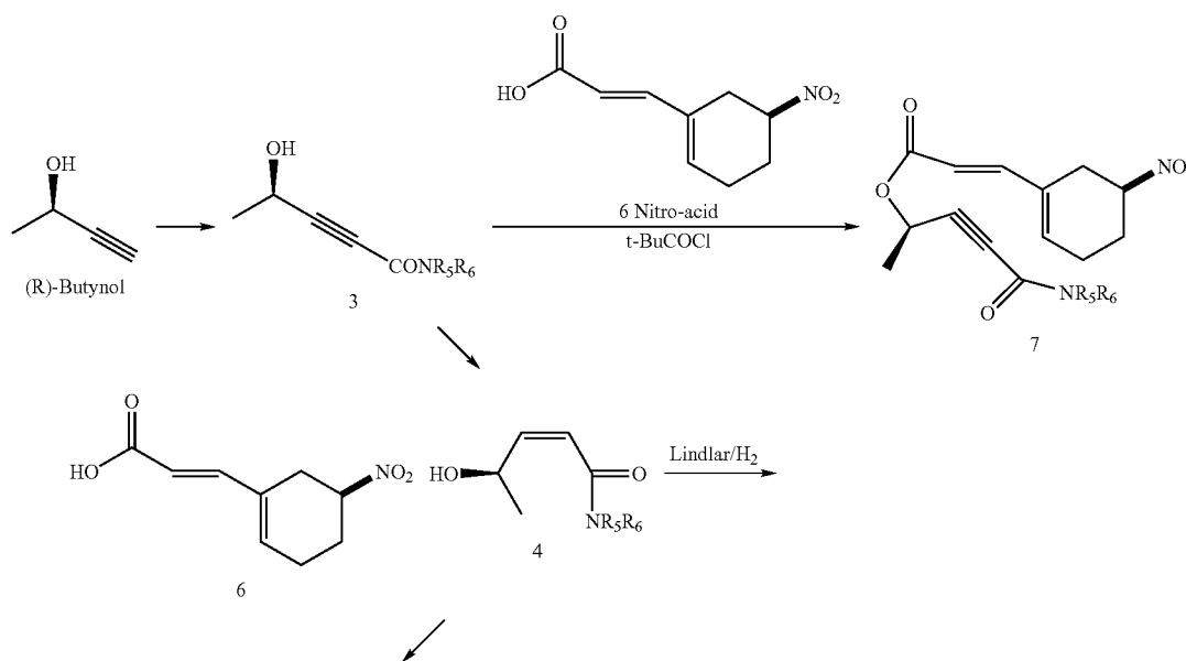
Scheme VII- the nitro-oxazole route for preparation of Compound 11:
