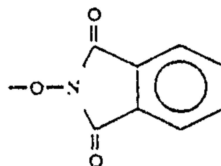
Oxyphthalimide
