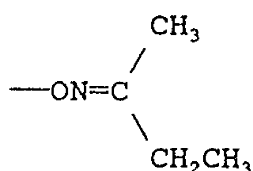
Methylethyl Ketoxime
