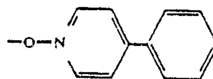
Phenylpyridinium N—Oxide
