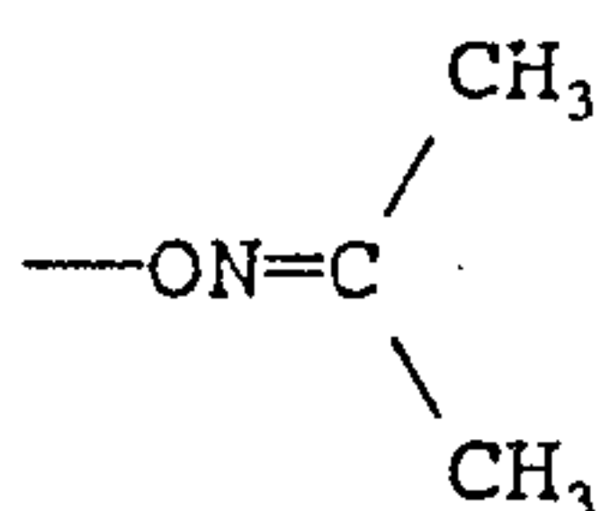
Acetone Oxime
