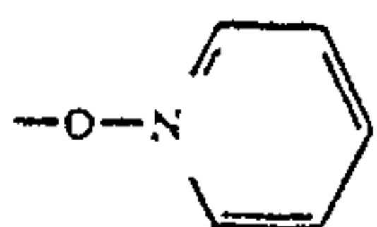
25 Pyridinium N—oxide
