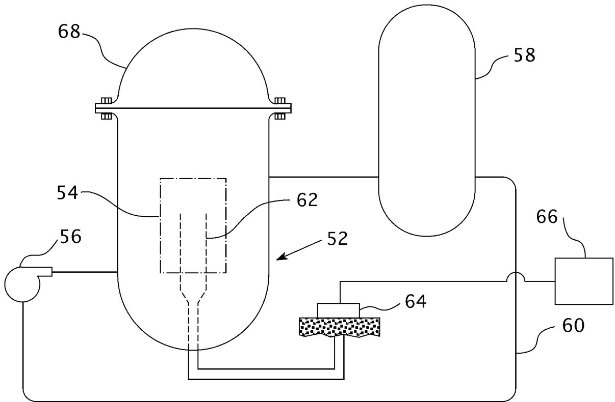
FIG. 3 Prior Art
