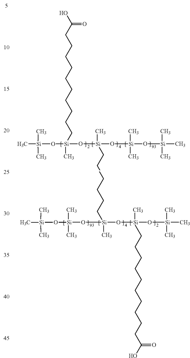
Example 7: Trimethylsilyl Undecylenate Elastomer Blend, De-Blocked
