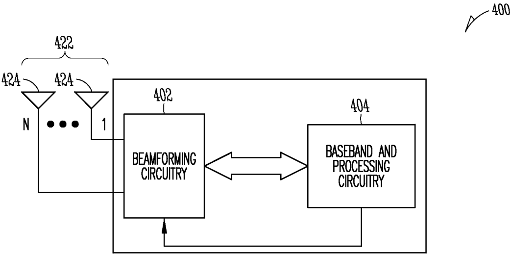
MILLIMETER-WAVE COMMUNICATION STATION
