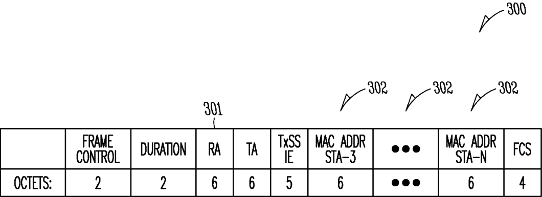
SECTOR SWEEP FEEDBACK FRAME
